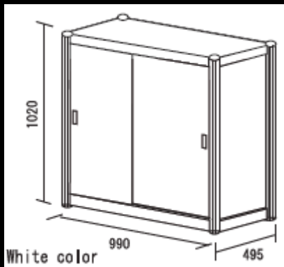
S-2 Display Counter w/ door & key
